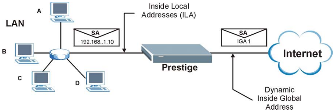
Figure 27-11 NAT Example 1
