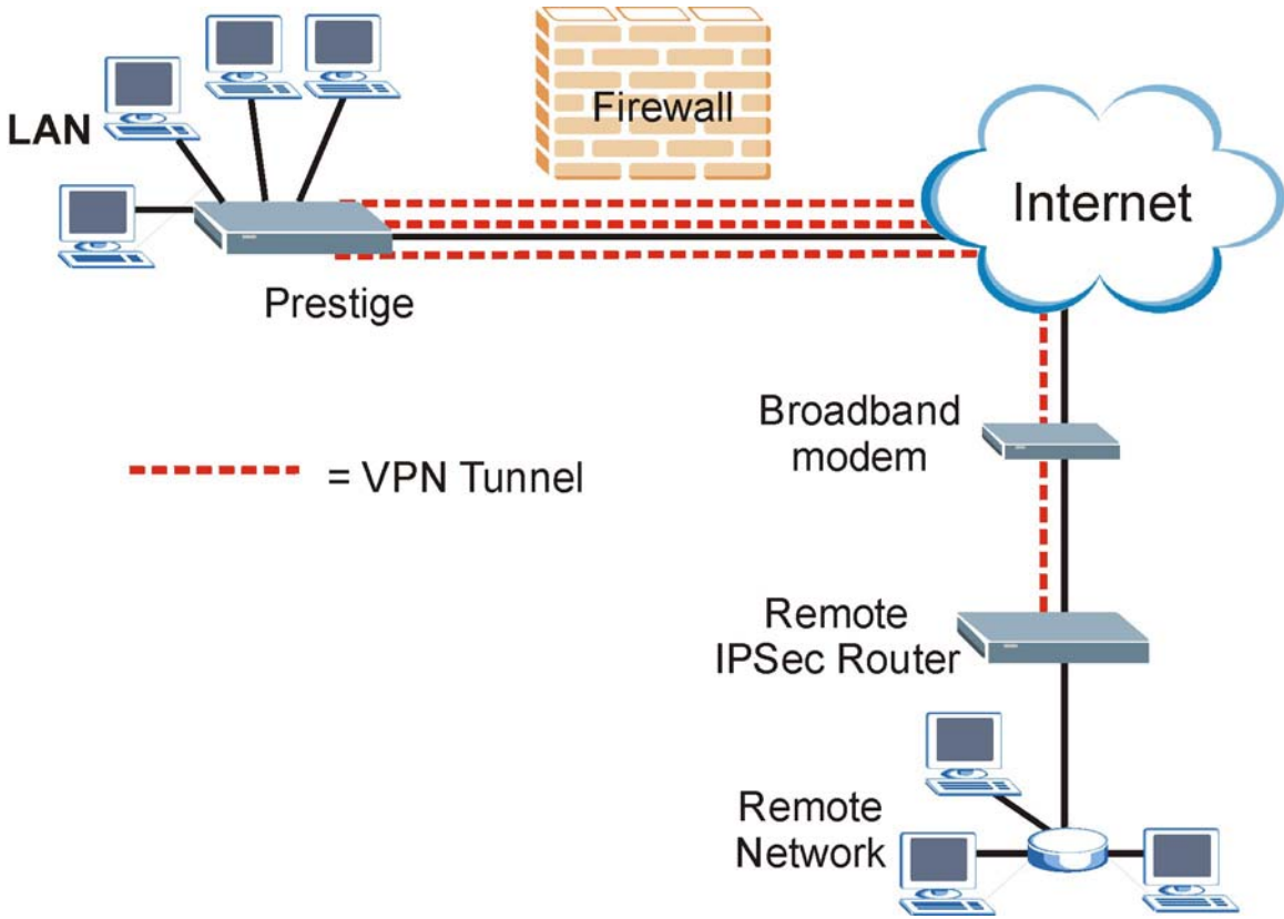
Figure 13-2 VPN Application
