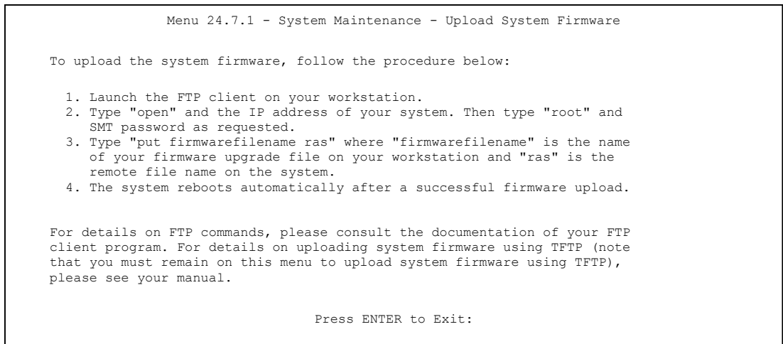
Figure 31-13 System Maintenance - Upload System Firmware
