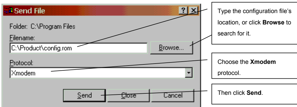
Figure 2-4 Example Xmodem Upload
