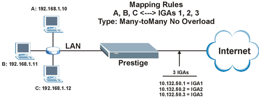
Figure 27-20 NAT Example 4
