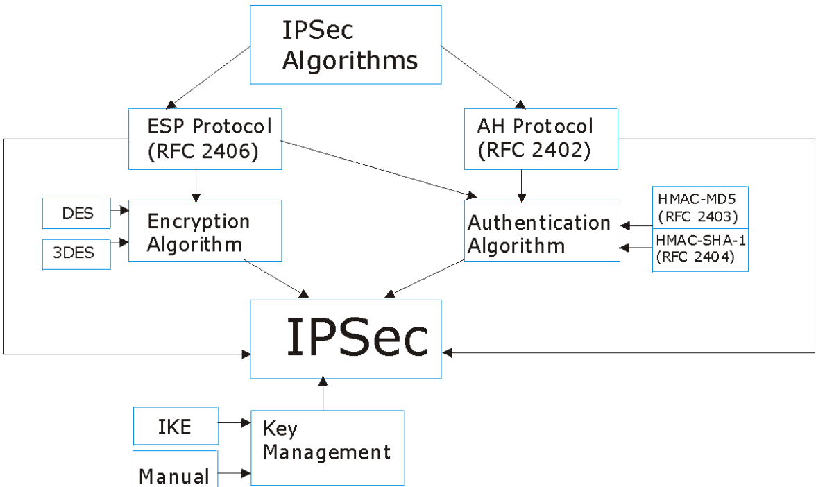
Figure 13-3 IPsec Architecture
